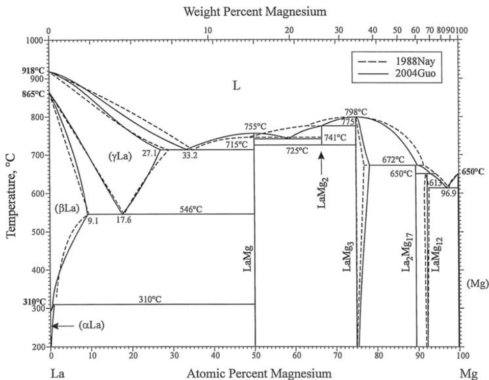
Fig. 1 La-Mg phase diagram
